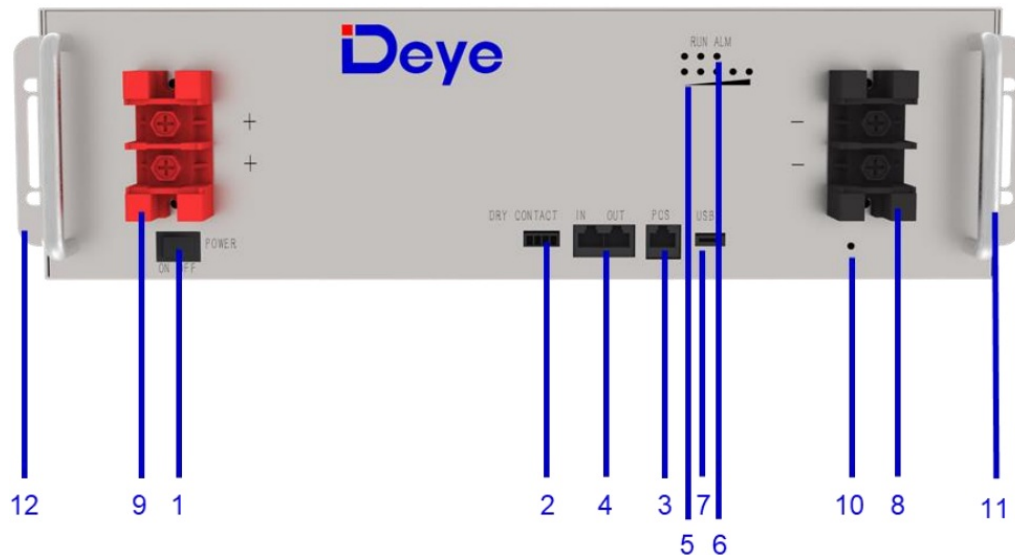
Figure 2-1: Front Panel Function Introduction
