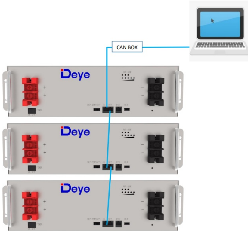
Figure 5-3: Communication Cable Connections between Battery and Computer
