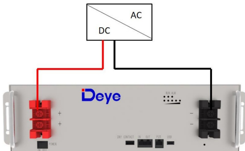
Figure 5-2: Single Battery Connection
